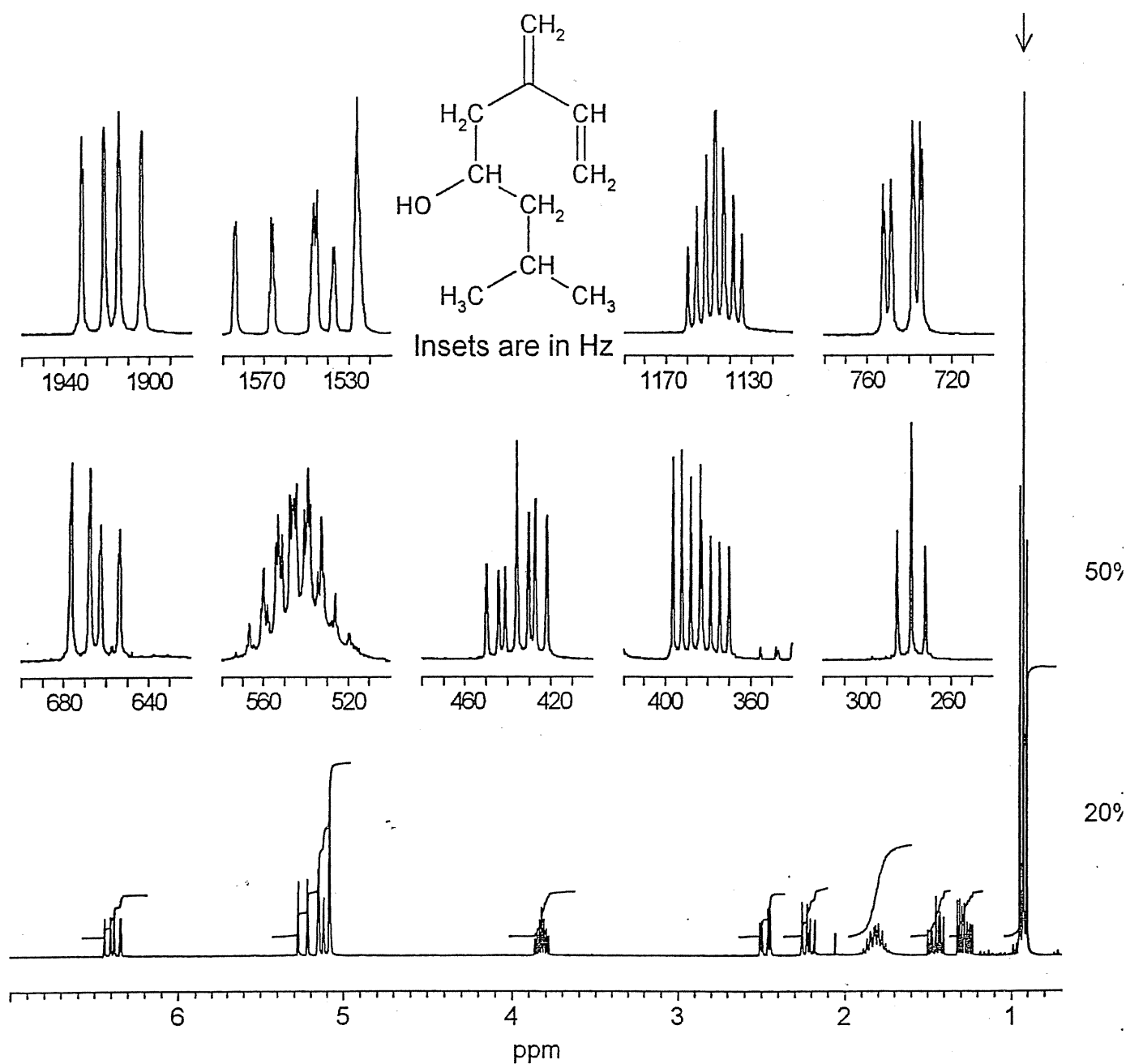
FIGURE 4.49. 2-Methyl-6-methylen-7-octen-4-ol (ipsenol) in \text{CDCl}_3 at 300 MHz. "Titration" with \text{C}_6\text{D}_6 . The sample was a gift from Phero Tech, Inc., Vancouver, BC, Canada.
