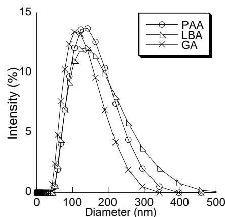
Figure 4. DLS plots of iron oxide nanoparticles coated with GA (cross), LBA (triangle), and PAA (circle).
