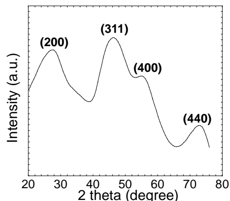
Figure 3. XRD scan of iron oxide nanoparticles.
